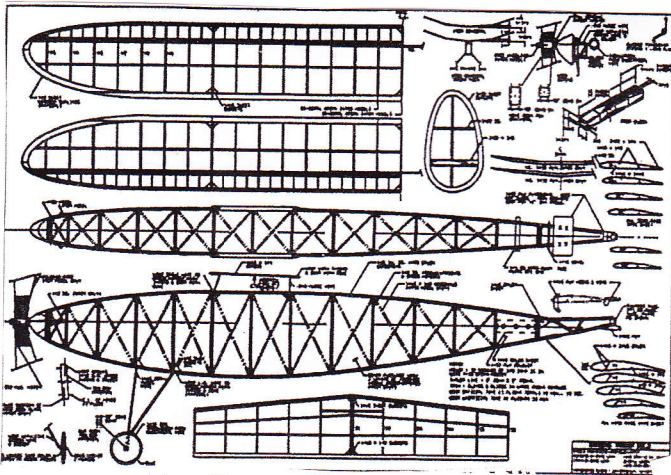
Linn, Kansas Champ, 1938
