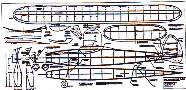
Struck, Flying Cloud, 1942
